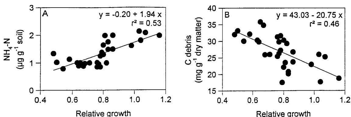
Figure 4. Relationships between relative growth and (A) \text{NH}_4\text{-N} or (B) C debris in Experiment 2. C debris is significantly negatively correlated and \text{NH}_4\text{-N} is significantly positively correlated with relative growth in Experiment 2 ( P < 0.05 ).
